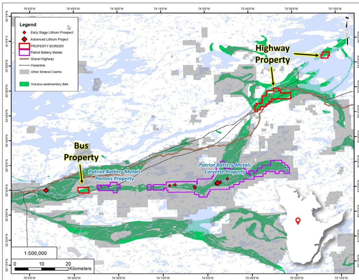
Figure 1. Norris Lithium's Highway and Bus Lithium Properties and other major lithium projects in the James Bay region of Québec.
